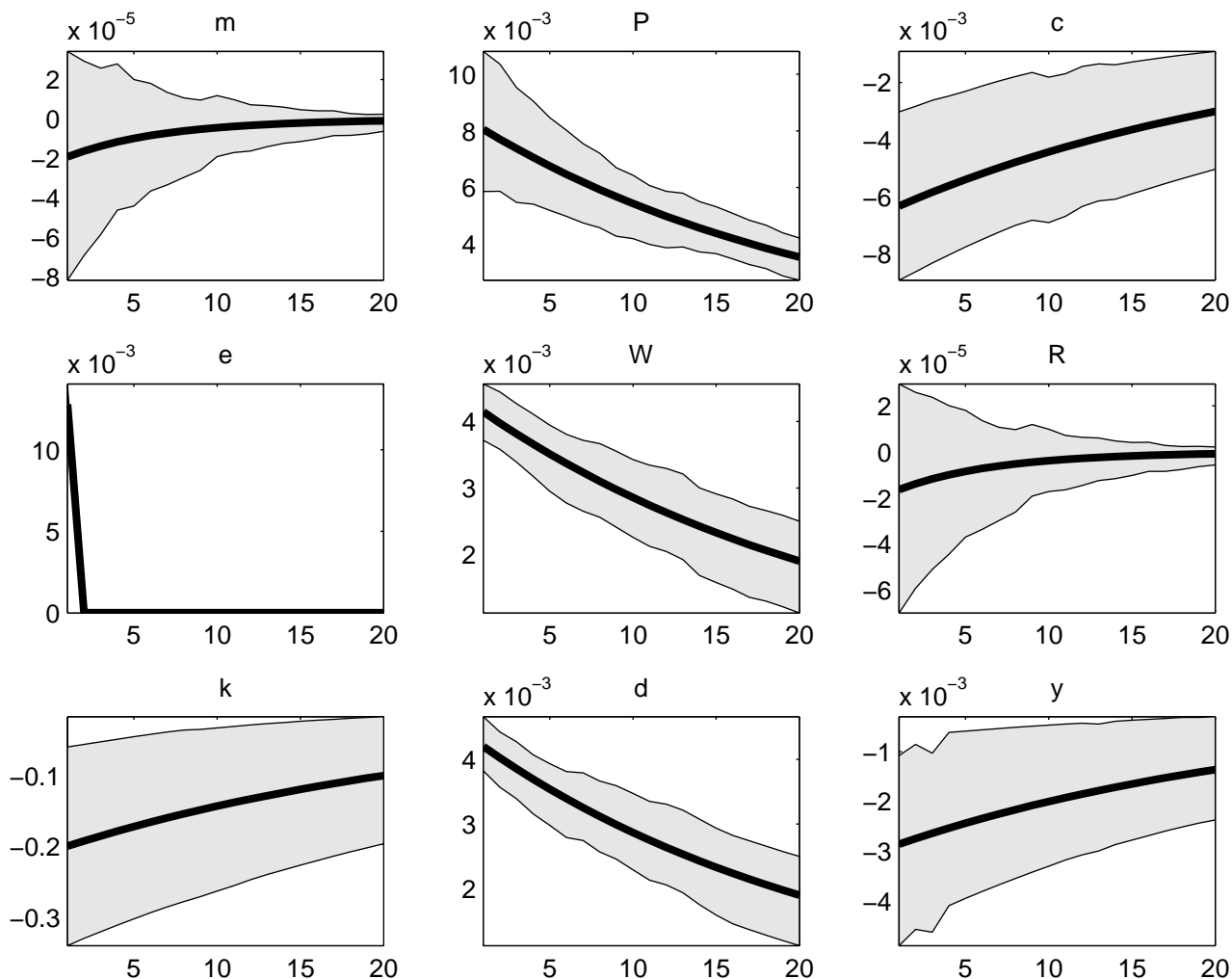
Figure 10: Orthogonalized shock to e\_a – Bayesian IRF plot generated by the bayesian_irf -option of the estimation -command. It is stored in the Output -subfolder. Generally, these IRFs are similar to the ones displayed in Figure 1 and use the same orthogonalization scheme. The main difference is that the stoch_simul -IRFs are computed at the calibrated parameter combination, while the Bayesian IRFs are the mean impulse responses (not to be confused with the IRFs at the mean). The gray shaded areas provide highest posterior density intervals (Highest Posterior Density Interval (HPDI)). If you want to compute classical IRFs after estimation, use stoch_simul after estimation as the latter will set the parameters to the posterior mode/mean, depending on whether you use maximum likelihood or Bayesian estimation. More information can be found in Adjemian, Bastani, Juillard, Karamé, Mihoubi, Perendia, Pfeifer, Ratto, and Villemot (2011)
