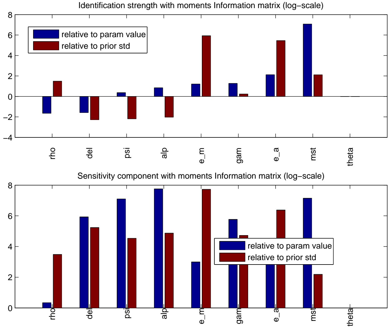
Figure 26: prior_mean - Identification using info from observables – Identification strength-plot generated by the identification -command. It is stored in the identification subfolder. Lower Panel: This panel further decomposes the effect shown in the upper panel. A weak identification can be due to either other parameters linearly compensating/replacing the effect of a parameter (i.e. parameters having exactly the same effect on the likelihood) or the fact that the likelihood does not change at all with the respective parameter. This latter effect is called sensitivity (computed according to formula (12) in Ratto and Iskrev (2011)) and is plotted in the bottom panel. Again, weighting can take place either with the prior mean (blue bars) or the prior standard deviation (red bars). The weighting with the prior standard deviation is only available if priors have been specified. For ML estimation, no blue bars will be displayed. The bottom panel shows that the sensitivity of theta is 0. Thus, theta is not identified at the local mean, because it does not affect the likelihood and hence the model moments.
