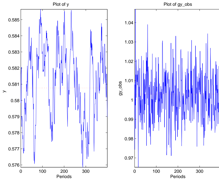
Figure 4: Simulated Trajectory – Plot of the simulated trajectory that can be generated by using the rplot -command after stoch_simul or simul . Graphs display the simulated series over the simulation horizon. When used with the option options_.rplottype=1 (top figure), the command prints one figure for each variable to plot. With option options_.rplottype=2 (bottom figure), the command prints all series into one figure, but with different subplots for each series. The graphs are saved in the graphs -subfolder.
